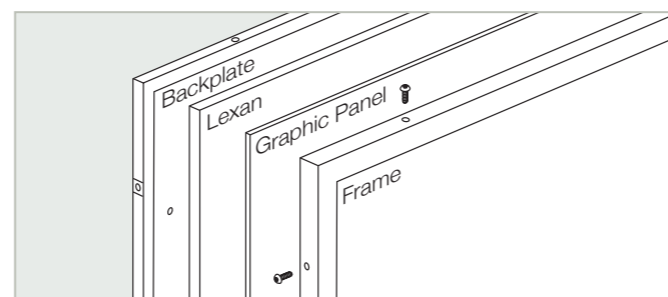
Standard assembly
