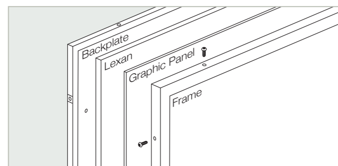
Standard assembly
